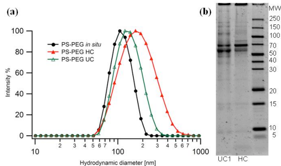
Fig. 3 HC complexes of PS-PEG. a) Size distribution by intensity percentage of PS-PEG NPs in situ 90% FBS (black dots), HC complexes isolated by centrifugation (HC, red triangles) and ultracentrifugation (UC, green empty triangles). b) SDS-PAGE gel of the HC complexes of PS-PEG NPs in 90% FBS isolated by ultracentrifugation (UC) and conventional centrifugation methods (HC), respectively, as indicated by the label below the tracks of the gel.
