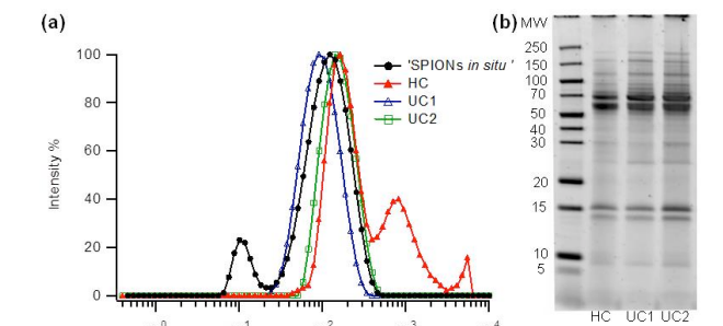
Fig. 5 Fe 3 O 4 in 55% FBS. a) Size distributions from DLS measures of Fe 3 O 4 NPs in situ and HC complexes recovered by ultracentrifugation (UC1-2) and by centrifugal washings (HC) b) SDS-PAGE of hard corona complexes isolated by conventional centrifugation (HC) and by density gradient ultracentrifugation (UC1-2).
